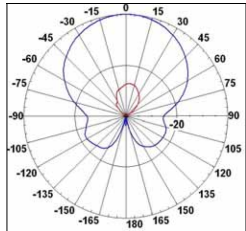
Elevation Radiation Pattern Midband Freq. 0.902 GHz
