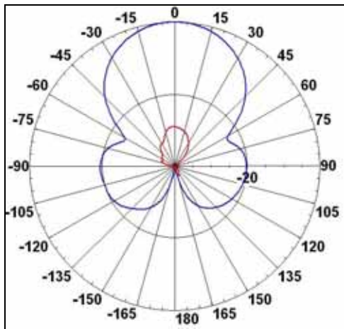
Azimuth Radiation Pattern Midband Freq. 0.902 GHz
